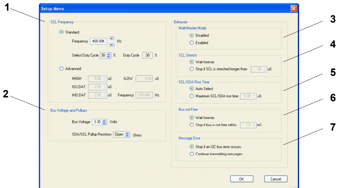
Figure 8. Setup Menu
